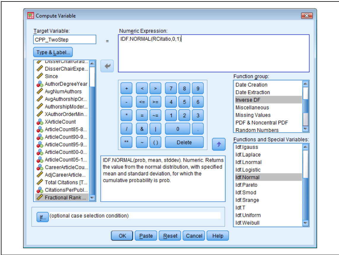
Figure 5. View of the Compute Variable Form in SPSS
